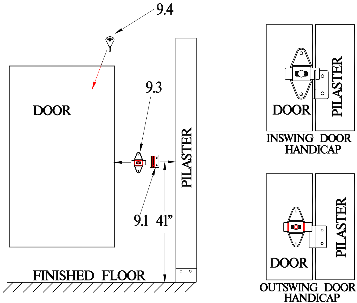
FIGURE 9.1 DOOR HARDWARE ATTACHMENT
